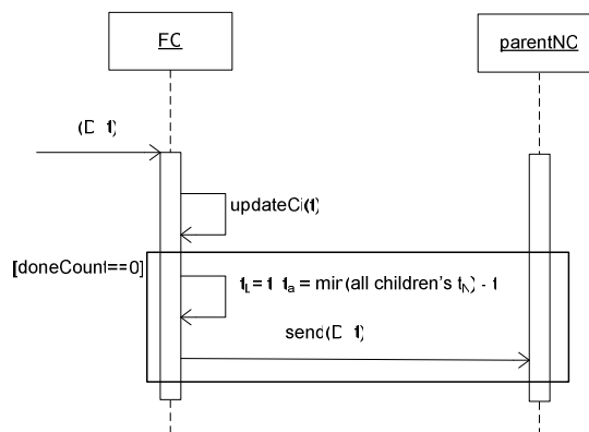
Figure 17. FC algorithm for (D, t)
