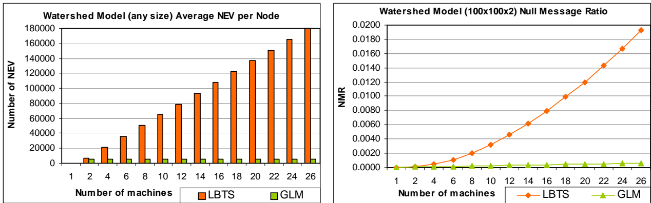
Figure 50. NMR Results of Watershed
