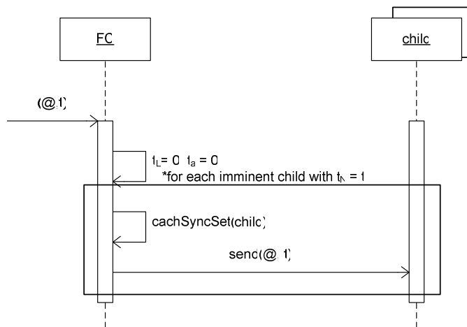
Figure 13. FC Algorithm for (@, t)
