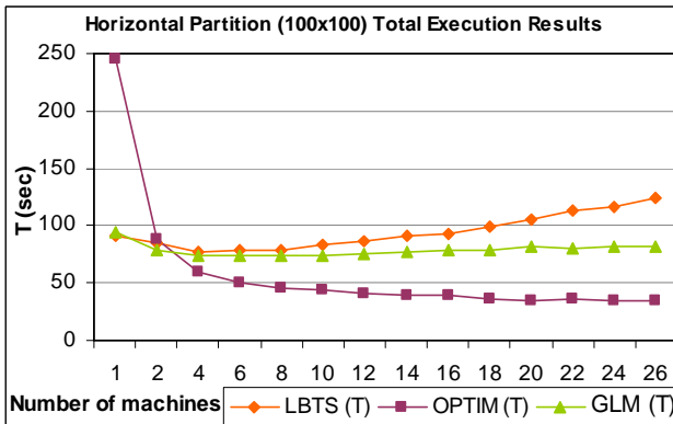
Figure 66. Partitioning Experiments of Fire2 Model (100x100)
