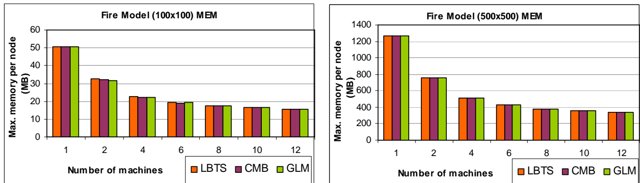
Figure 53. Fire1 Model Memory Consumption Results
