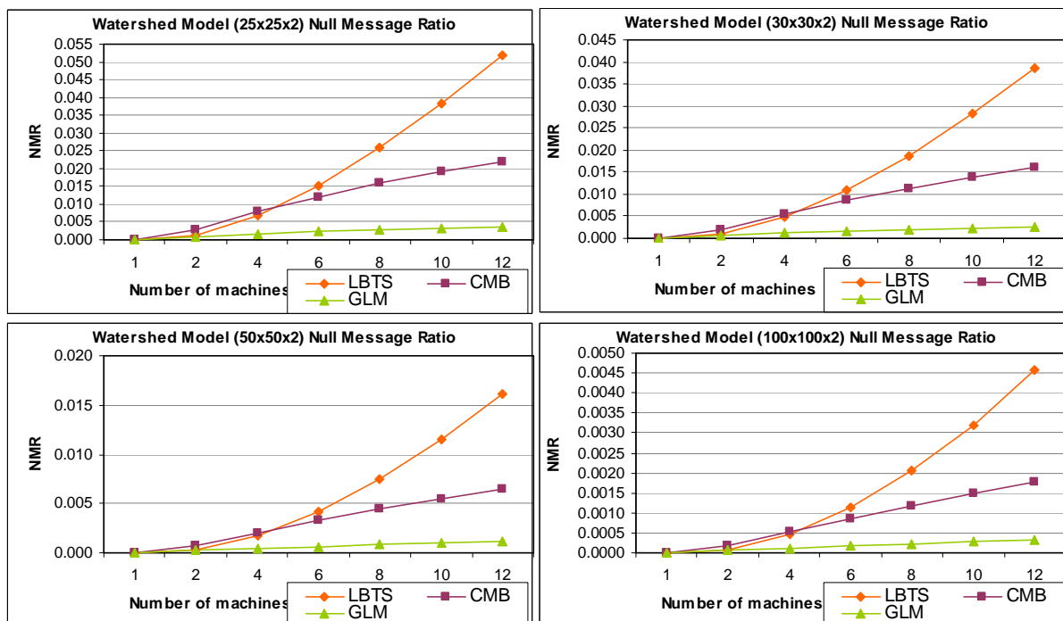
Figure 58. Watershed Model NMR Results
