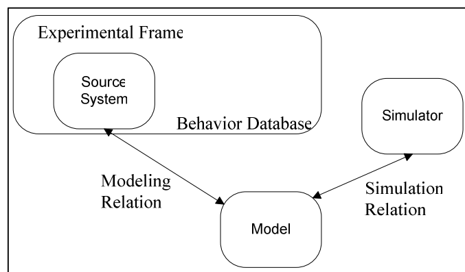
Figure 1. Entities and Relationships of a System M&S Framework [8]
