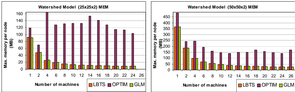
Figure 51. Memory consumption for Watershed model
