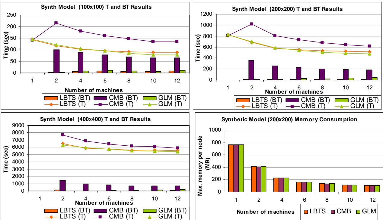
Figure 56. Synth Model Results
