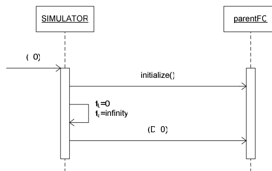
Figure 8. Simulator Algorithm for (I, 0)
