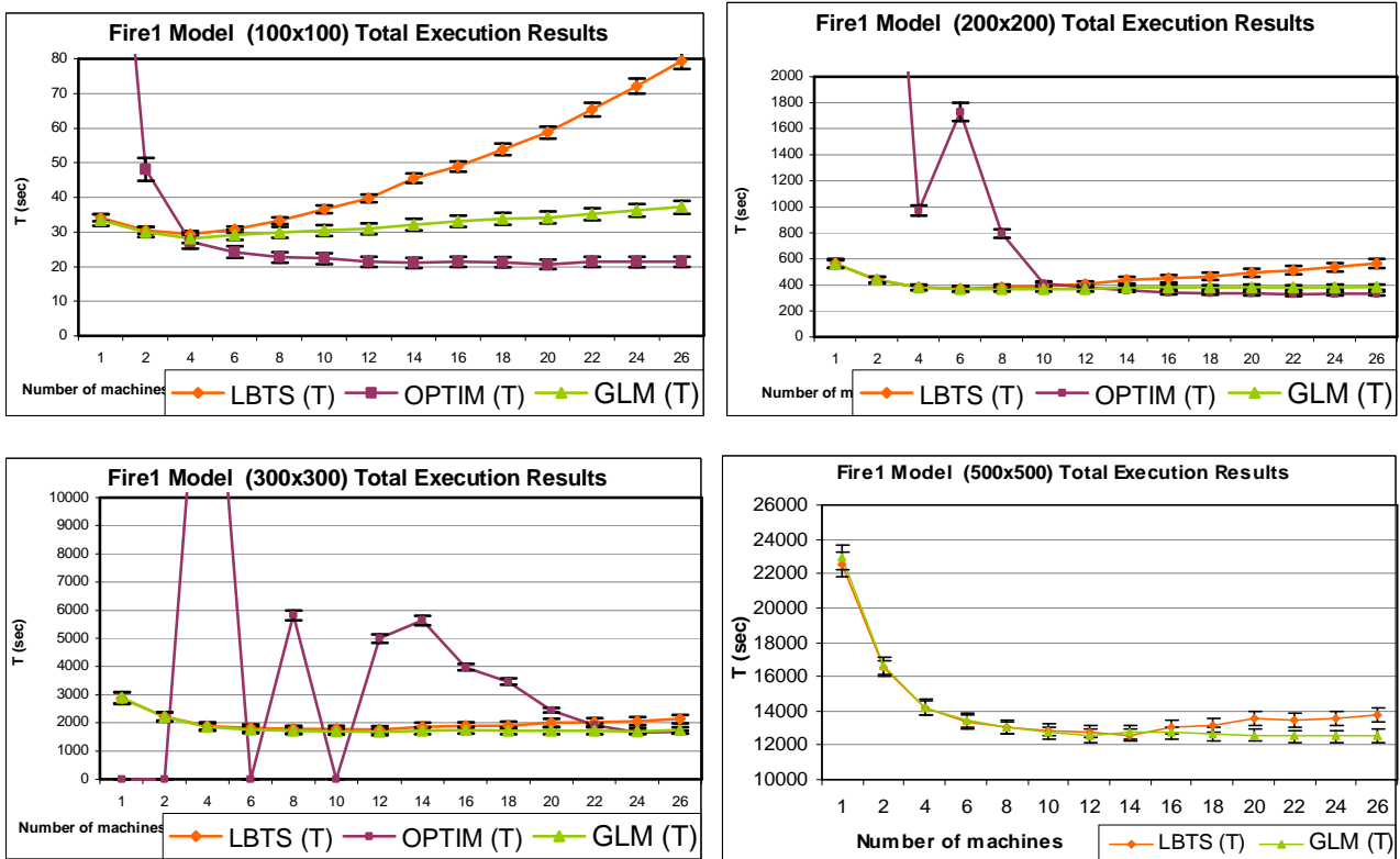
Figure 40. Fire1 Results for Various Sizes
