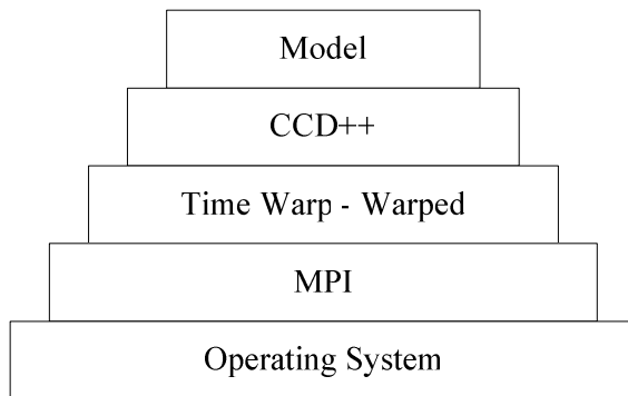
Figure 6. Layered Architecture of CCD++ Simulator [21]
