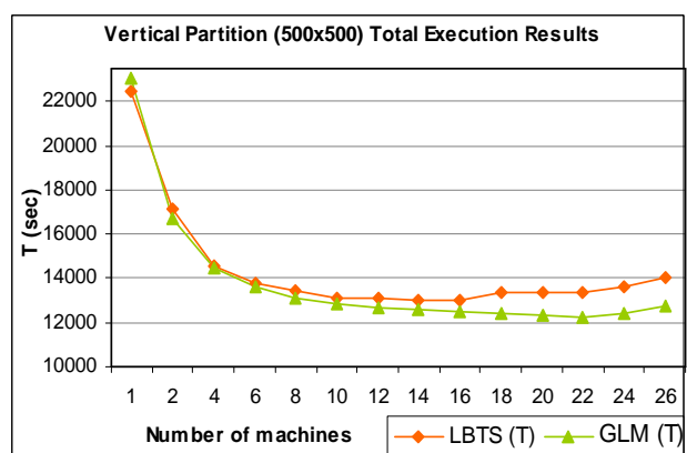
Figure 65. Partitioning Experiments of Fire1 Model (500x500)
