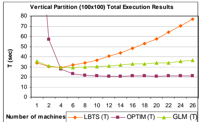
Figure 63. Partitioning Experiments of Fire1 Model (100x100)
