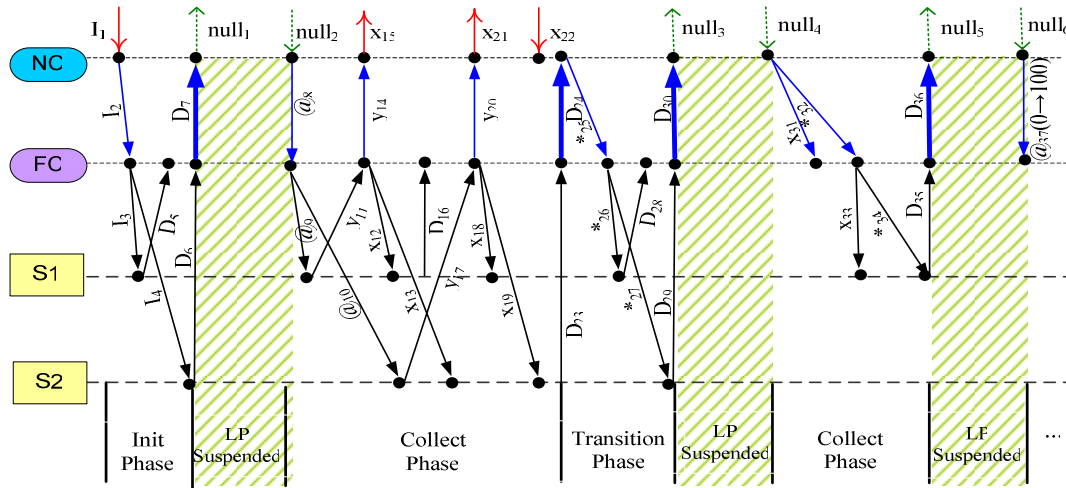
Figure 28. Sample Simulation Scenario in CCD++
