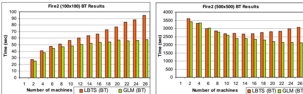
Figure 45. BT Results of Fire2
