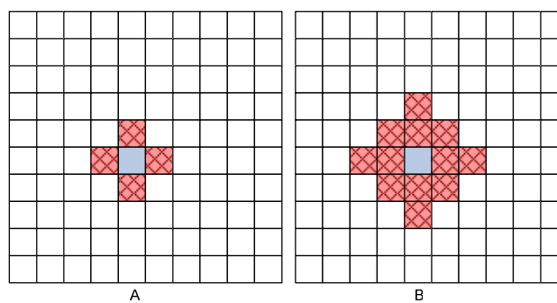
Figure 33. A: Small, and B: Large Cell Neighborhood
