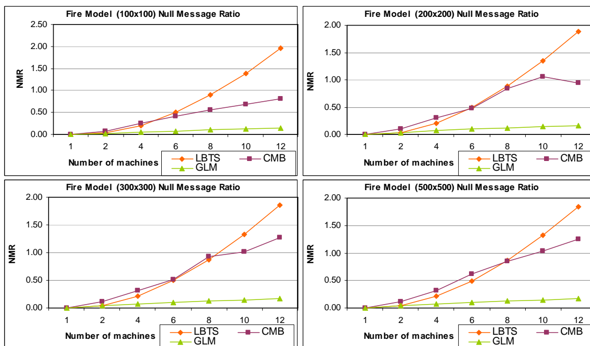
Figure 57. Fire1 Model NMR Results
