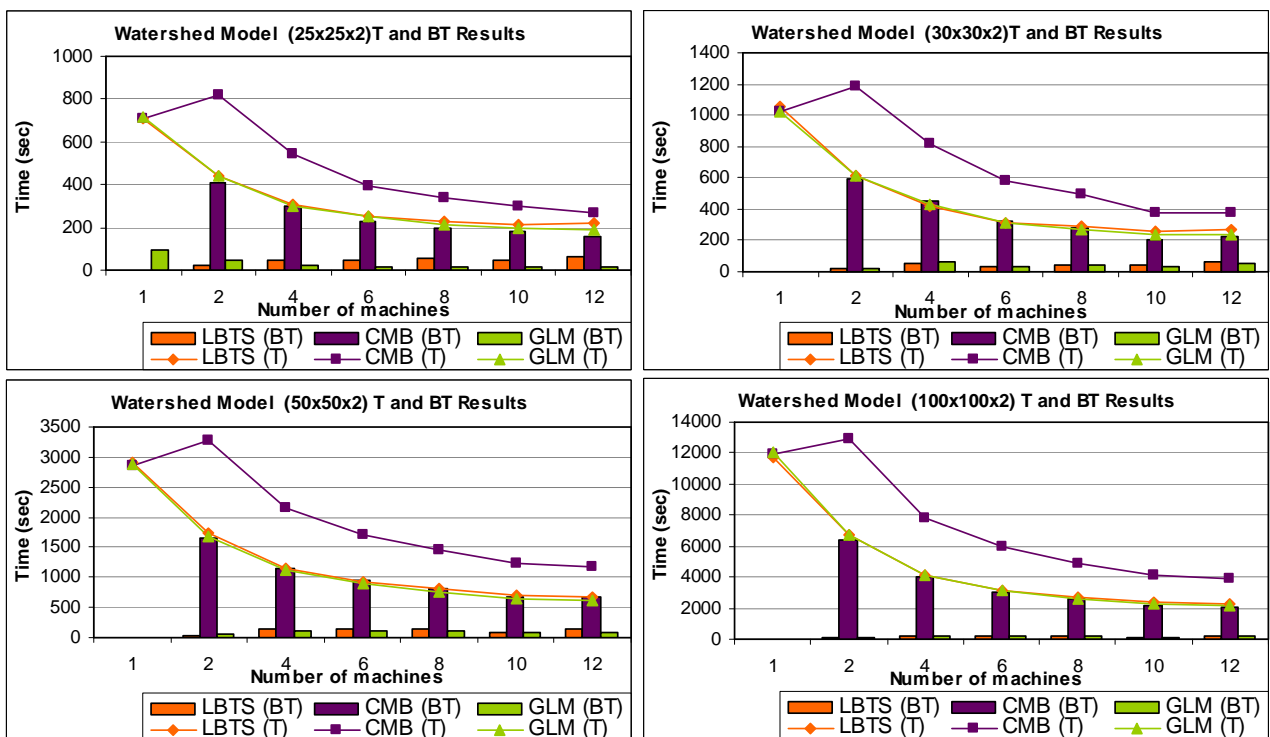
Figure 54. Watershed Model T and BT Results
