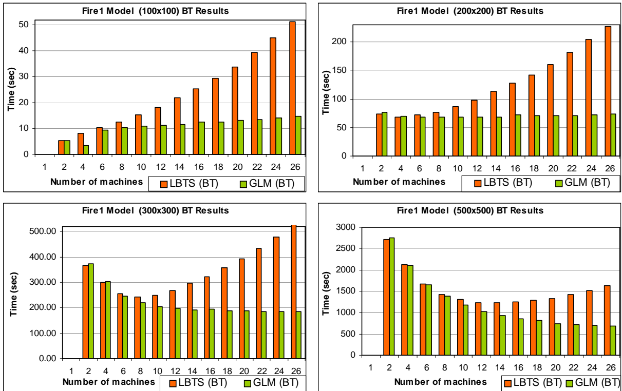
Figure 41. BT Results of Fire1
