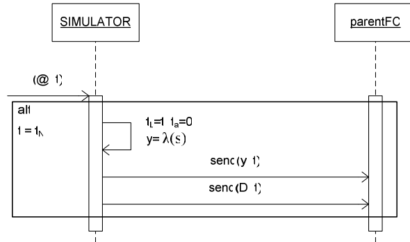
Figure 9. Simulator Algorithm for (@, t)
