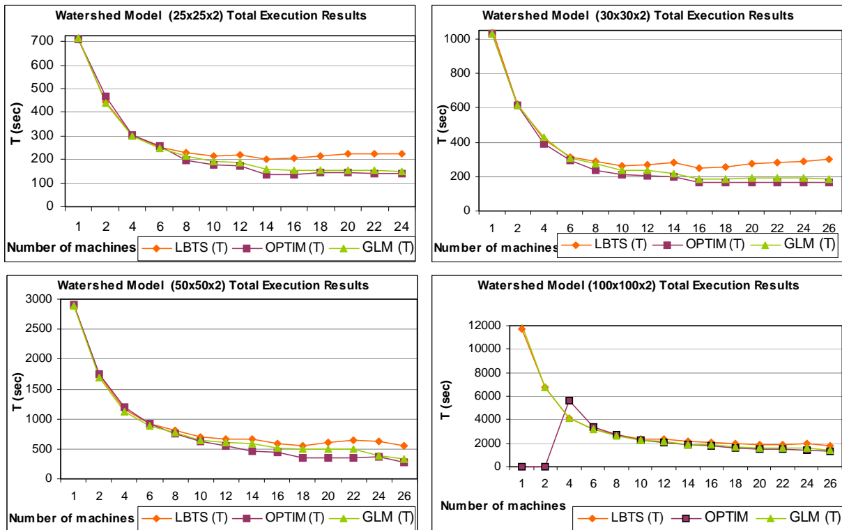
Figure 48. Watershed Results for Various Sizes
