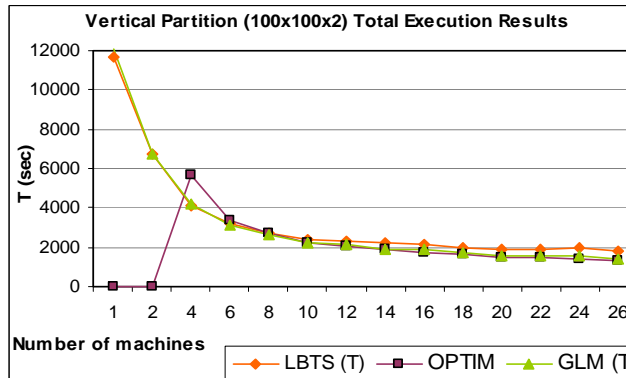
Figure 71. Partitioning Experiments of Watershed Model (100x100x2)
