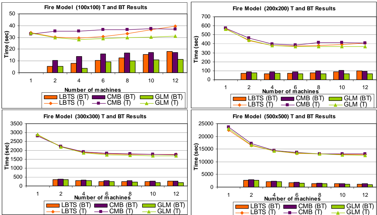
Figure 52. Fire1 Model T and BT Results
