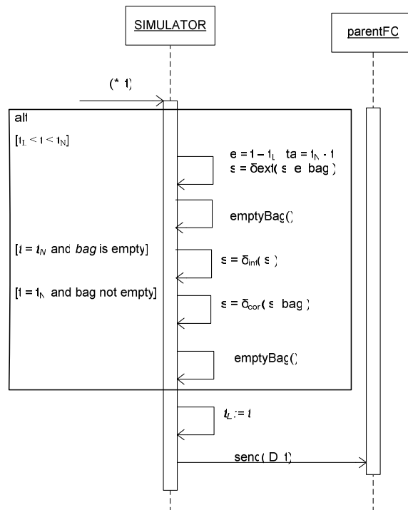
Figure 10. Simulator Algorithm for (*, t)
