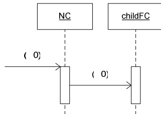
Figure 18. NC algorithm for (I, 0)
