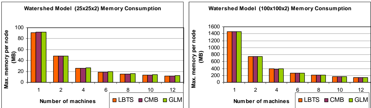
Figure 55. Watershed Model Memory Consumption Results
