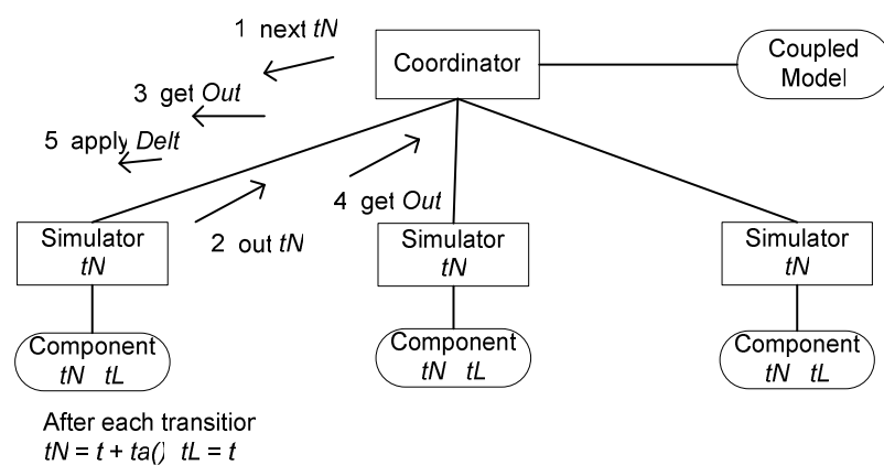
Figure 30. Parallel DEVS Simulation Protocol [82]
