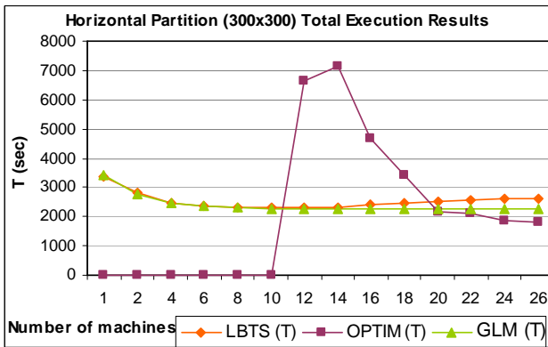
Figure 67. Partitioning Experiments of Fire2 Model (300x300)
