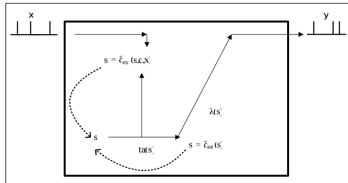
Figure 2. DEVS Semantics of an Atomic Model [8]
