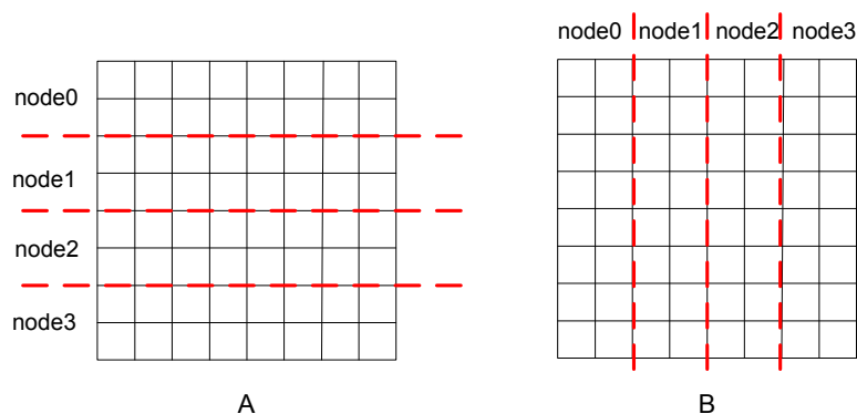
Figure 32. A: Horizontal, B: Vertical Partitioning of an 8x8 Cell-DEVS Model on Four Nodes
