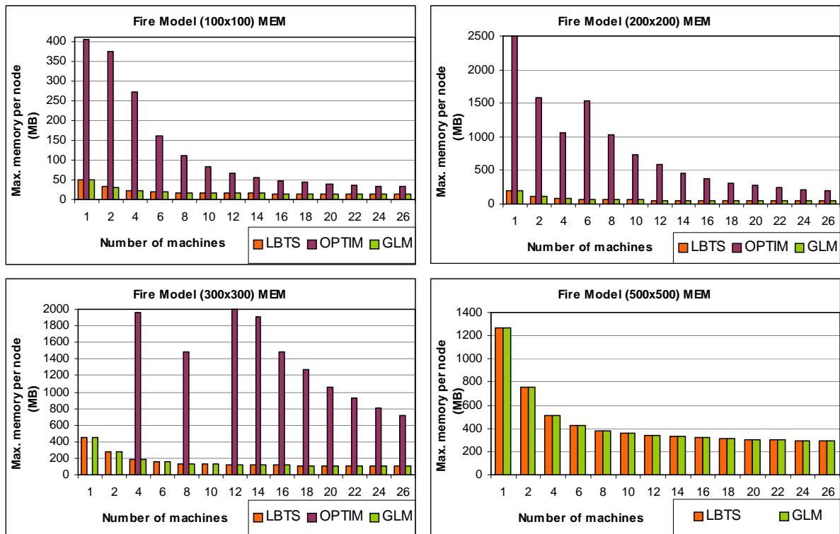
Figure 43. Memory Consumption for Fire1 Model
