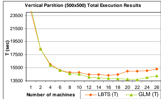
Figure 68. Partitioning Experiments of Fire2 Model (500x500)
