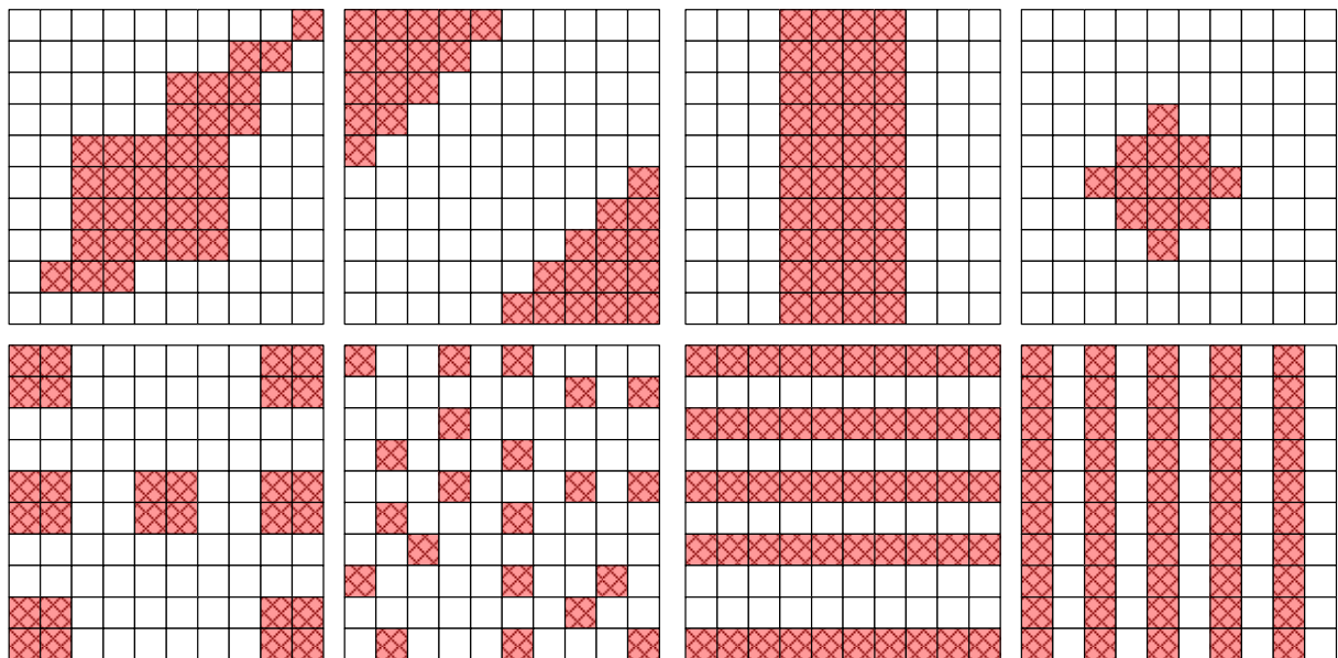
Figure 31. Sample Activity Patterns in Cell-DEVS Models
