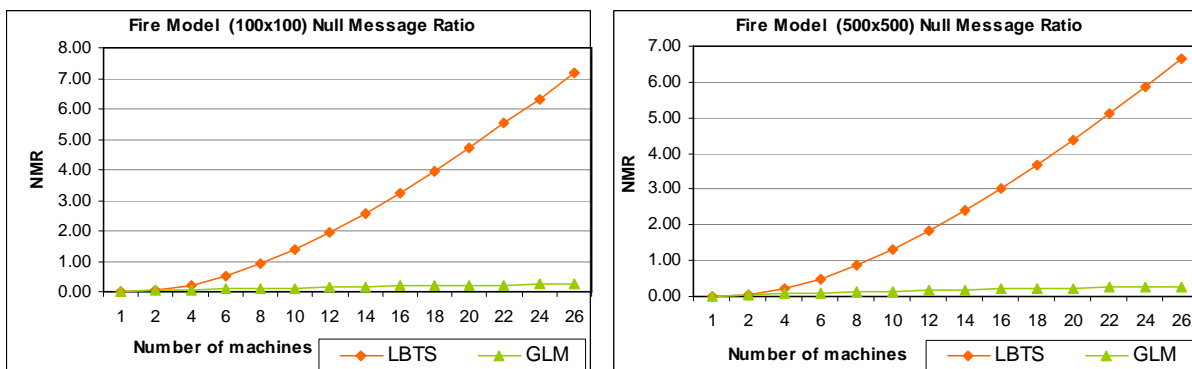
Figure 46. NMR Results of Fire2
