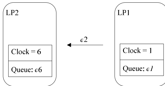
Figure 5. Causality Error Scenario
