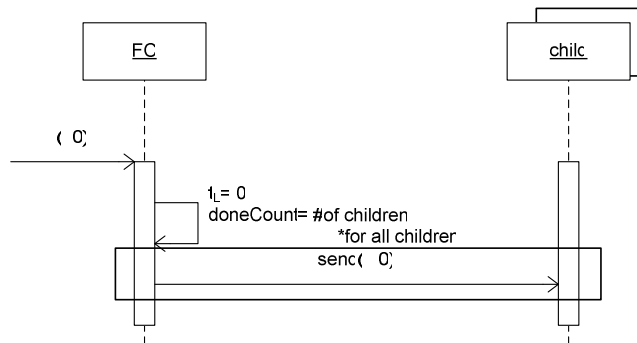
Figure 12. FC Algorithm for (I, t)
