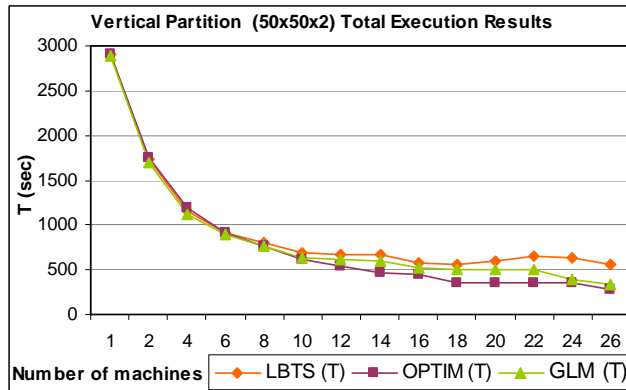
Figure 70. Partitioning Experiments of Watershed Model (50x50x2)
