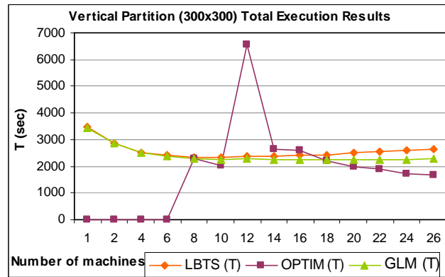
Figure 67. Partitioning Experiments of Fire2 Model (300x300)
