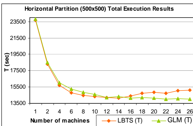
Figure 68. Partitioning Experiments of Fire2 Model (500x500)
