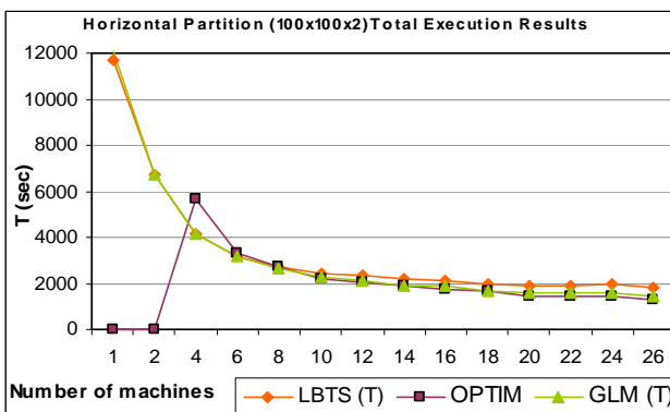
Figure 71. Partitioning Experiments of Watershed Model (100x100x2)
