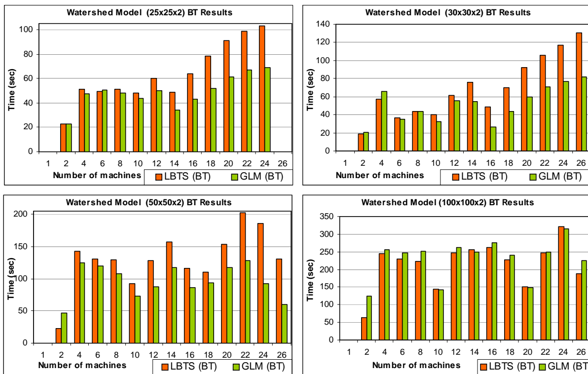
Figure 49. BT Results of Watershed
