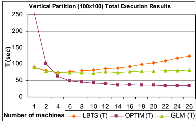
Figure 66. Partitioning Experiments of Fire2 Model (100x100)
