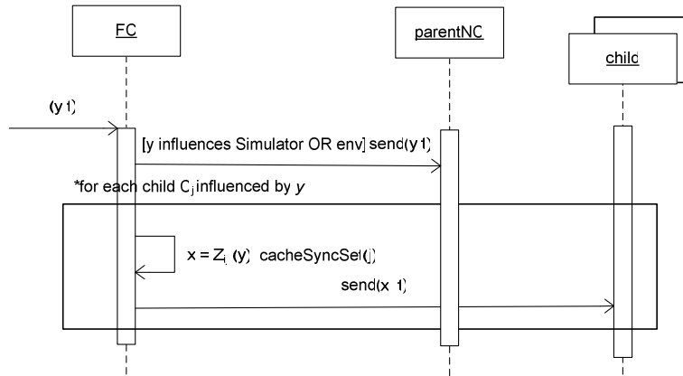
Figure 14. FC Algorithm for (y, t)
