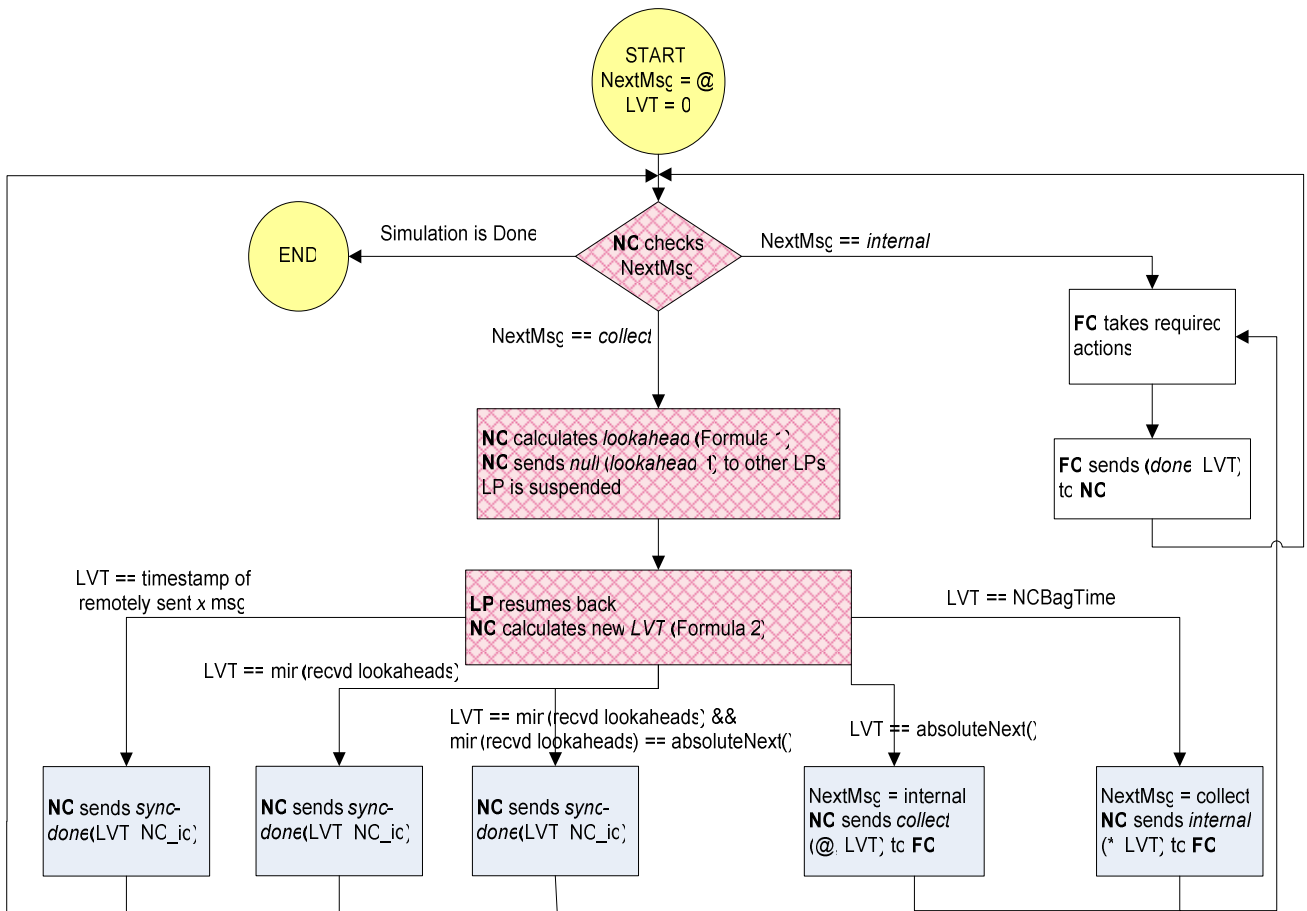
Figure 22. Flow Chart of the Conservative Algorithm on each LP
