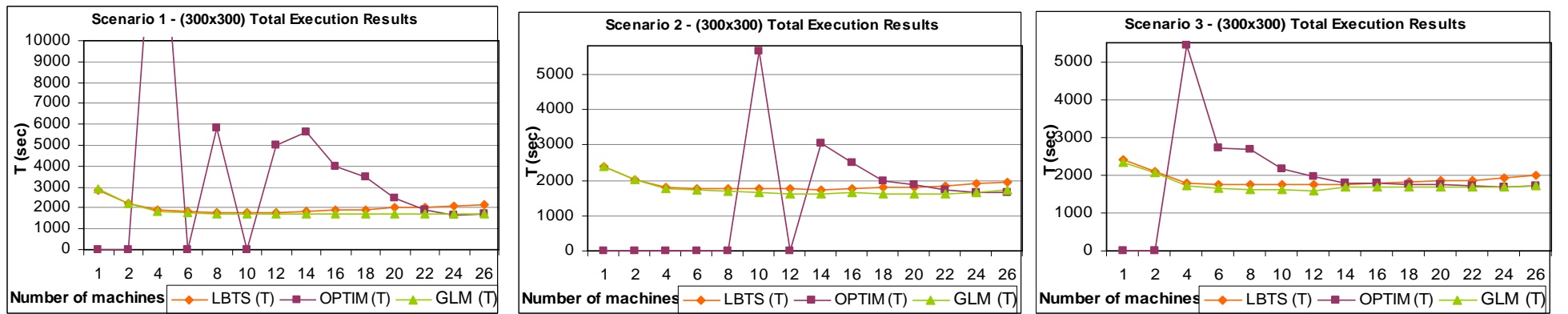
Figure 61. Initial States Analysis of FireI Model (300x300)
