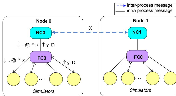
Figure 7. CCD++ Flat Architecture and Message-Passing Paradigm
