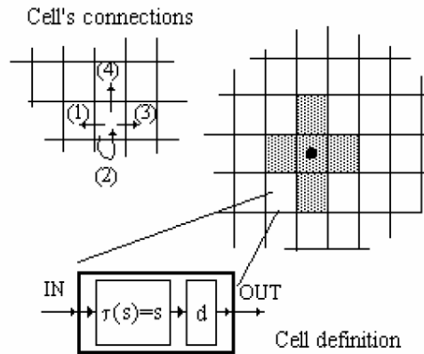
Figure 4. A Timed Cell-DEVS Atomic Model [100]
