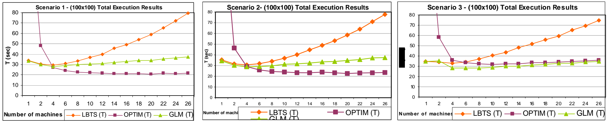
Figure 60. Initial States Analysis of FireI Model (100x100)
