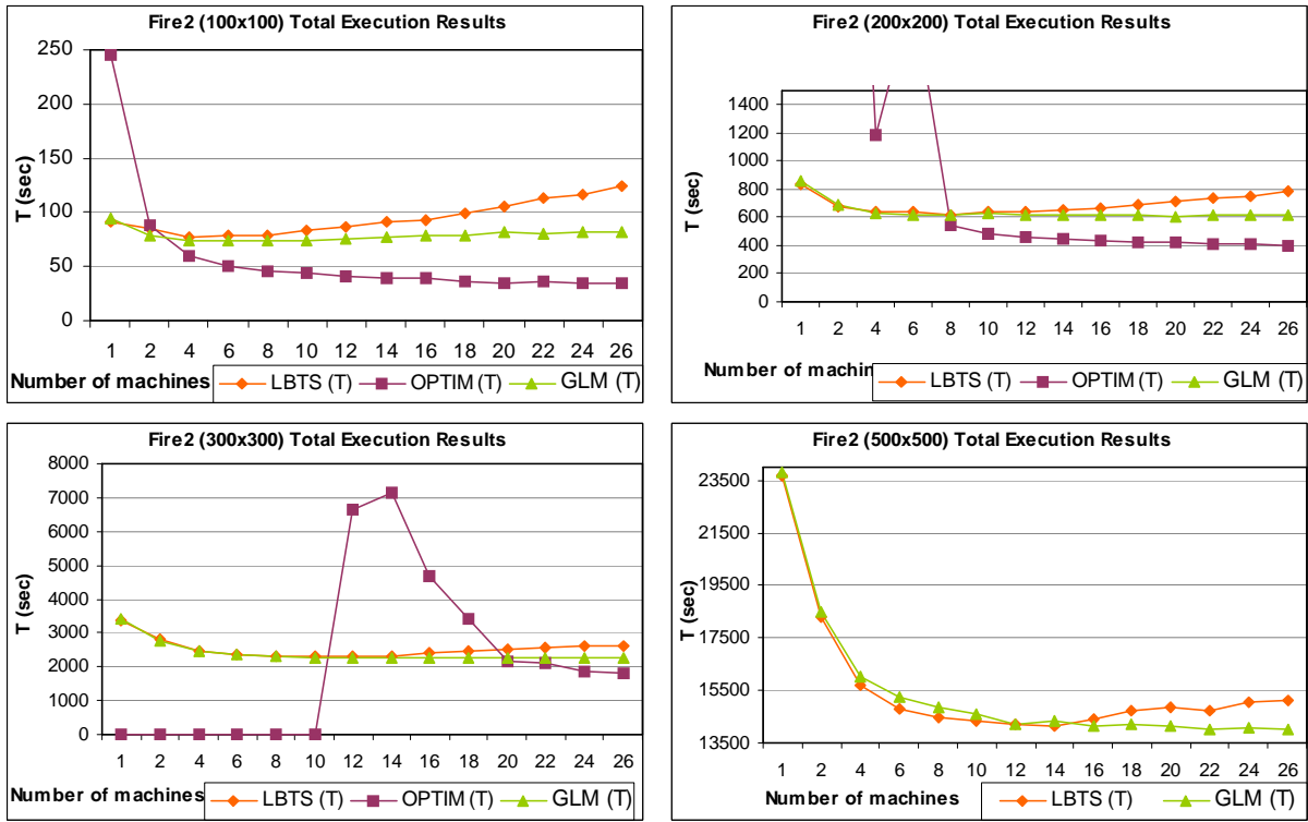
Figure 44. Fire2 Results for Various Sizes
