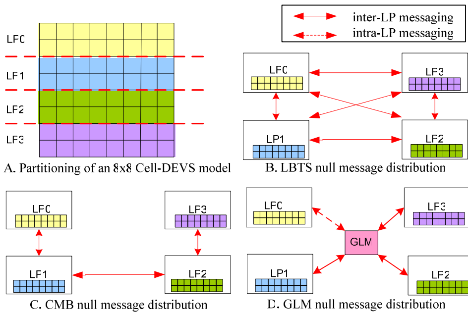
Figure 29. Null Message Distribution Strategy in LBTS, CMB, and GLM Protocol
