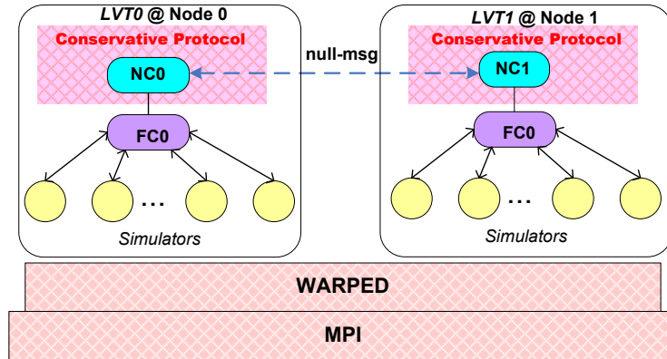
Figure 21. Conservative Architecture of CCD++
