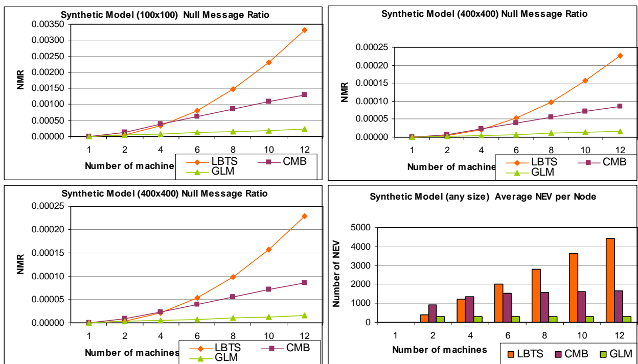
Figure 59. Synth Model NMR and NEV Results
