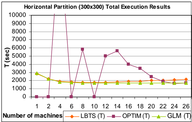
Figure 64. Partitioning Experiments of Fire1 Model (300x300)
