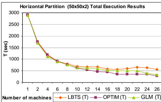
Figure 70. Partitioning Experiments of Watershed Model (50x50x2)
