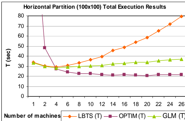
Figure 63. Partitioning Experiments of Fire1 Model (100x100)
