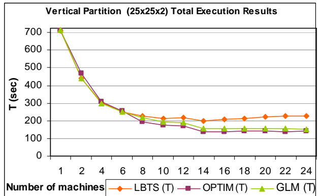
Figure 69. Partitioning Experiments of Watershed Model (25x25x2)
