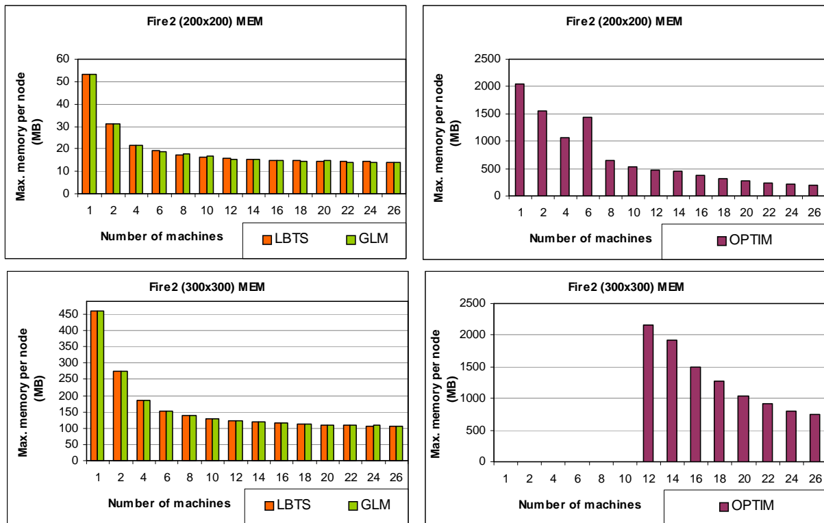
Figure 47. Memory Consumption for Fire2 Model
