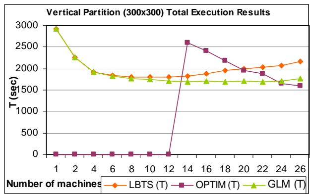
Figure 64. Partitioning Experiments of Fire1 Model (300x300)
