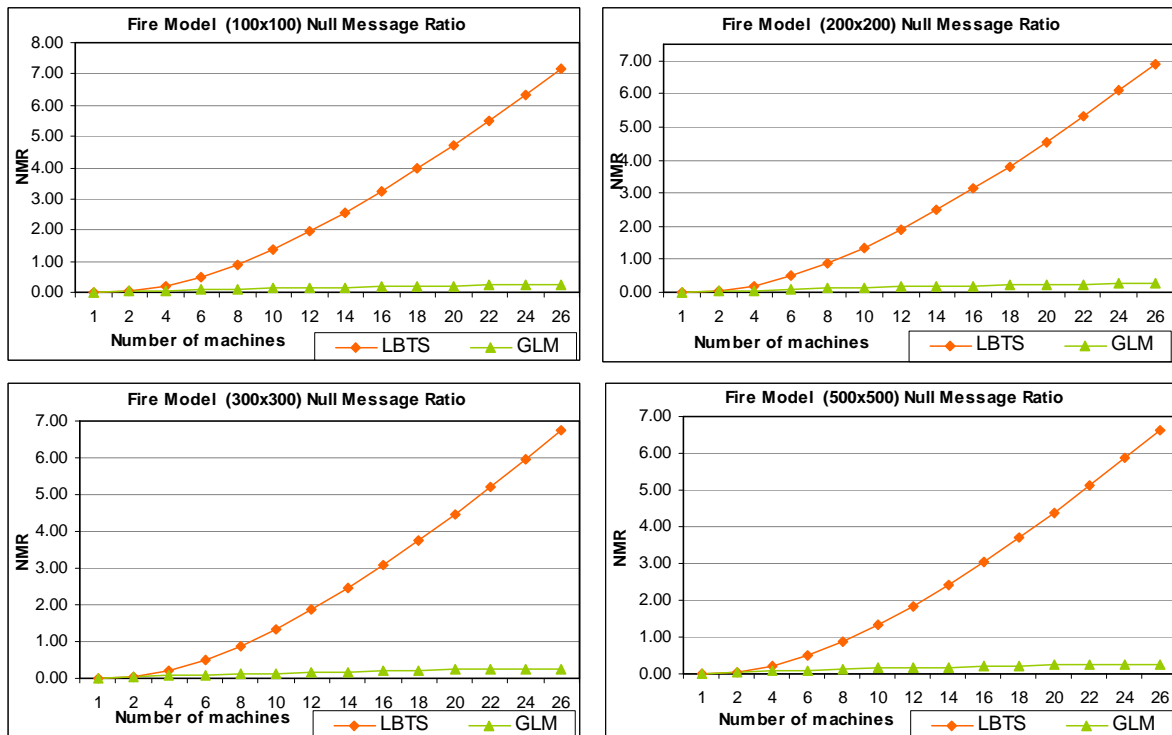
Figure 42. NMR Results of Fire1
