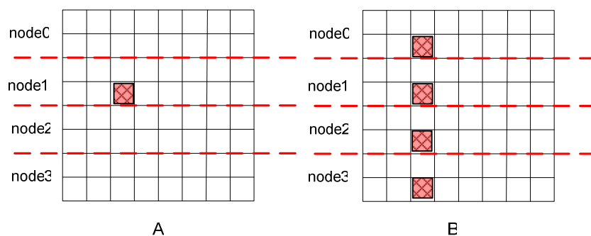
Figure 34. Initial-Load Distribution by Setting Multiple Initial Points
