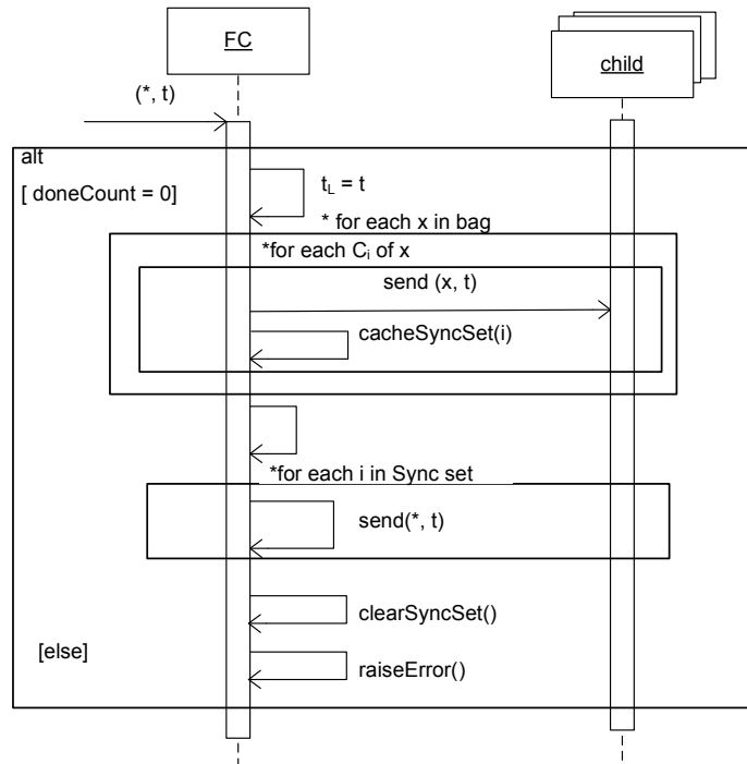
Figure 16. FC Algorithm for (*, t)
